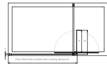
Foldaway Deflector
