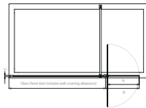
Hinged Deflector
